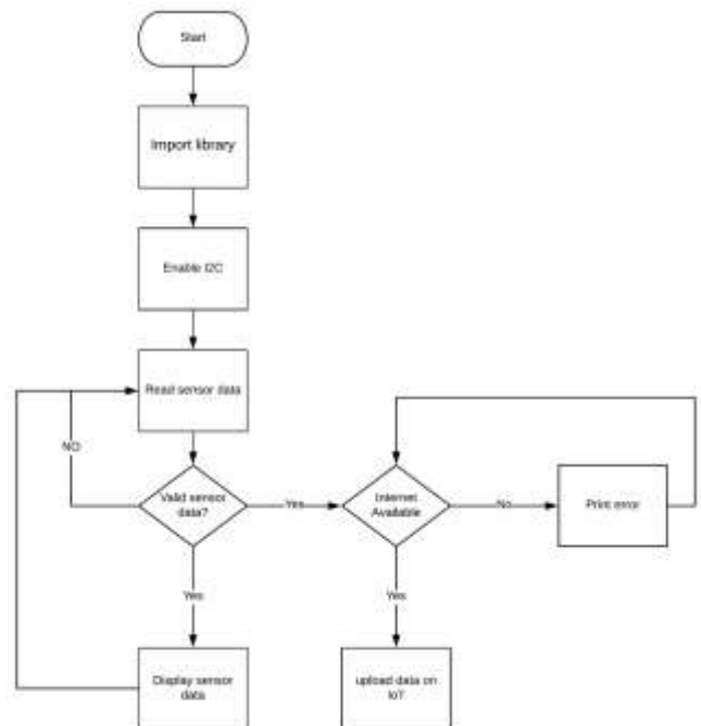
Fig. 5. Flow chart of proposed system
