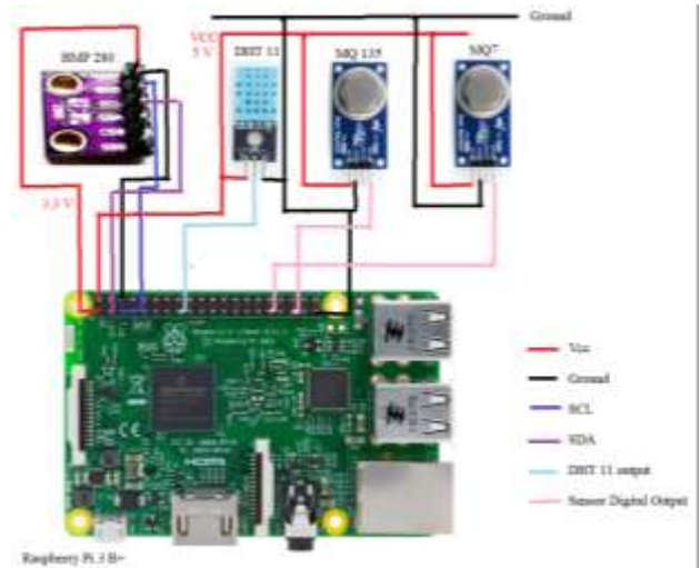
Fig. 4. Circuit diagram of proposed system
