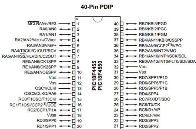
Fig. 3 PIC18F4550
