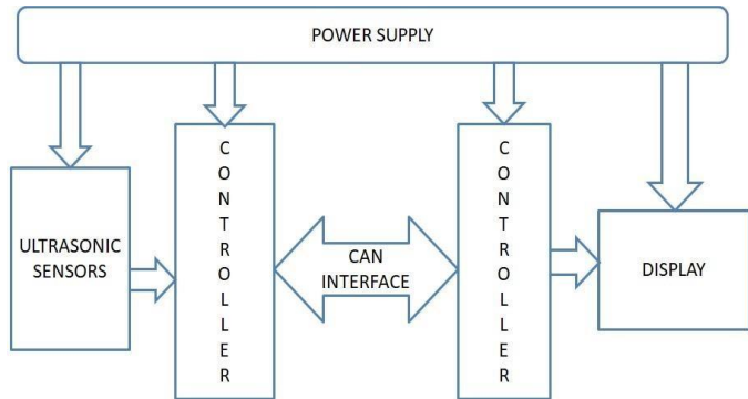
Fig. 2 Block diagram
